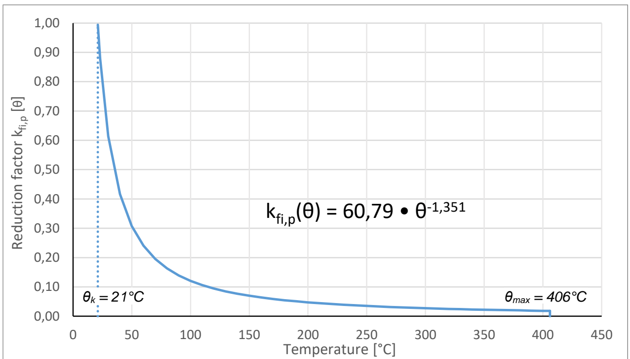
Figure C1: Reduction factor k_{fi,p}(\theta)
