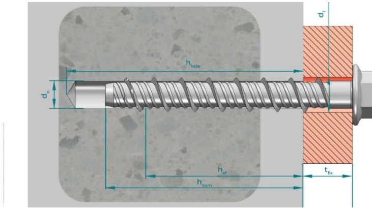
FIGURE 1—ANCHOR DIMENSIONS
