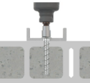
FIGURE 3—MANUFACTURER’S PUBLISHED INSTALLATION INSTRUCTIONS
